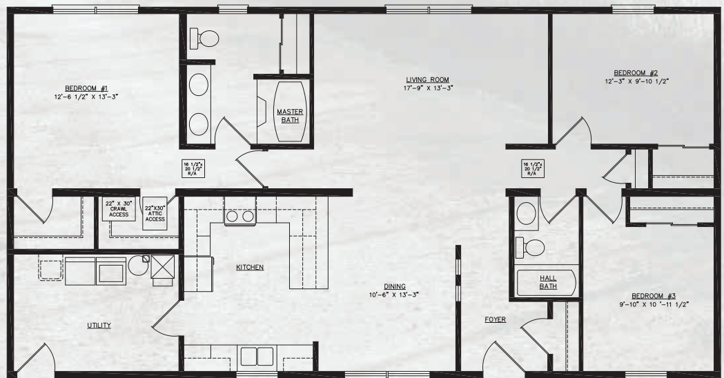
CRAWLSPACE PLAN
