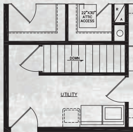
BASEMENT PLAN
