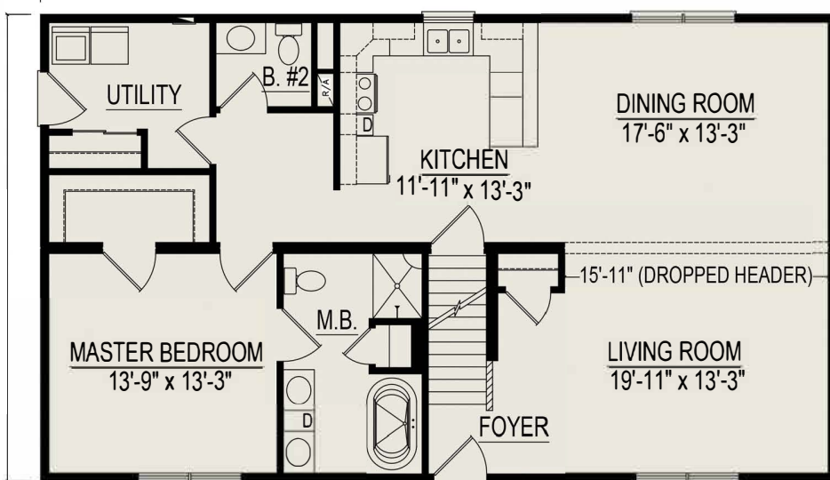
1st Floor Basement Plan
